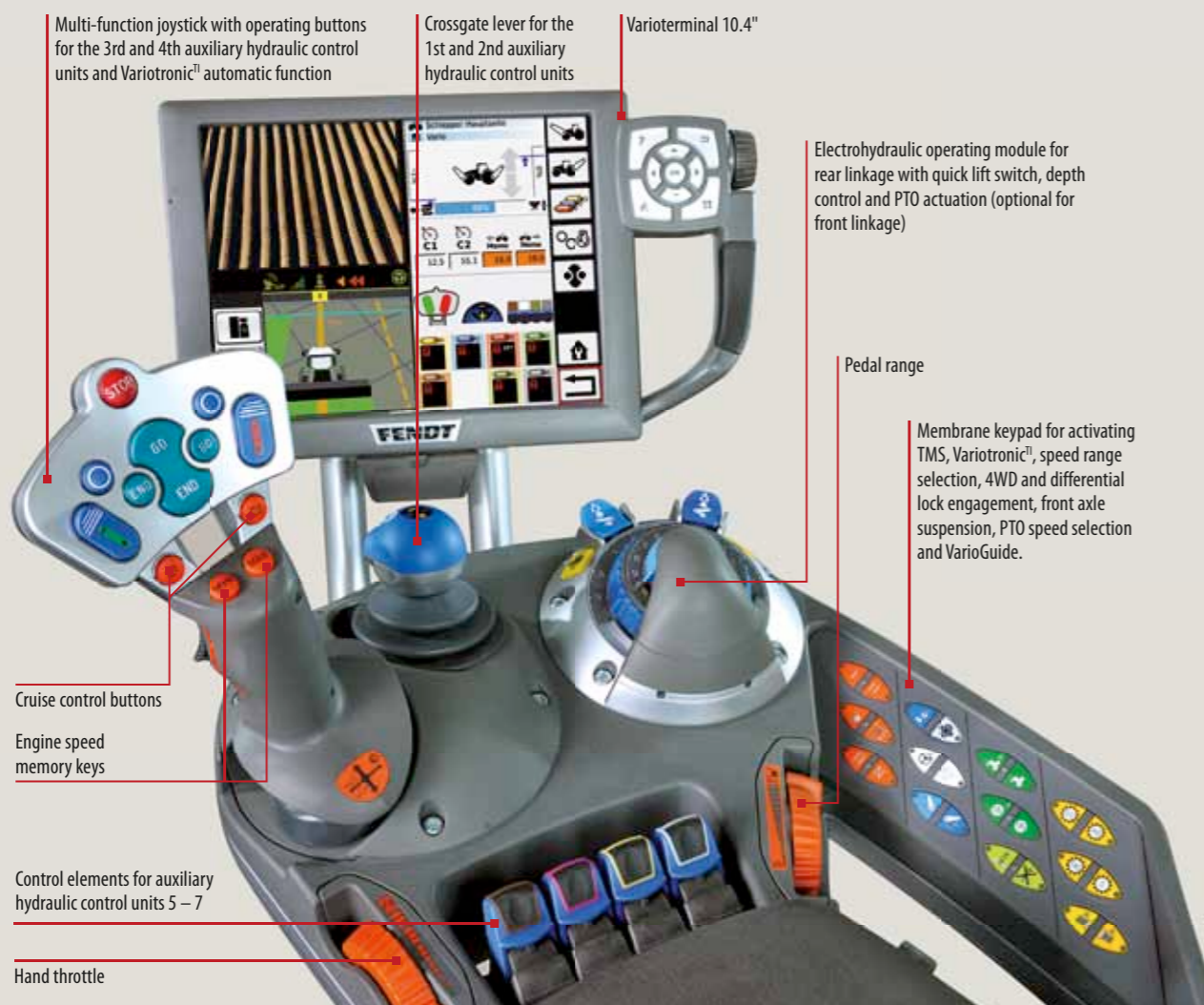
Control via keys or touch
