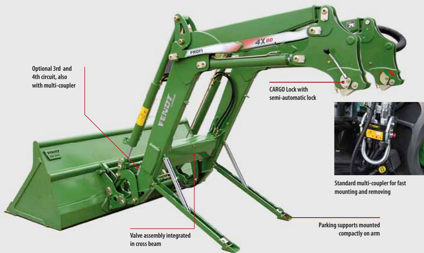
Torsion-resistant arm for rugged jobs
