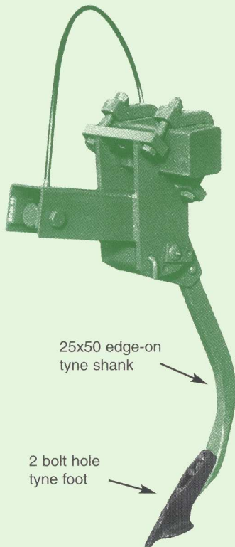
Model 800H Hydraulic Tyne (P/N 37124)
